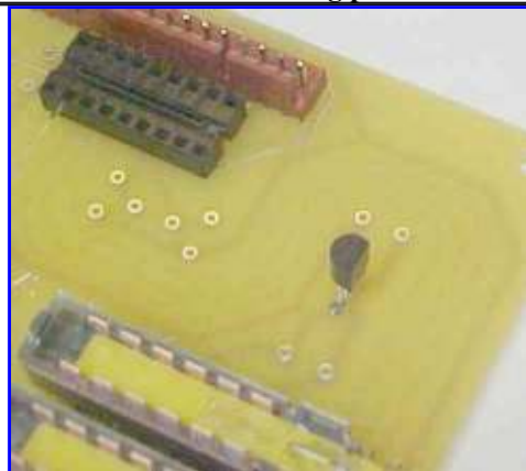
Install the voltage regulator flat side toward right
